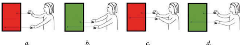
FIGURE 1 The Mathematical Imagery Trainer for Proportion set at a 1:2 ratio, so that the favorable sensory stimulus (a green background) is activated only when the right hand is twice as high along the monitor as the left hand. This figure sketches out our Grade 4–6 study participants' paradigmatic interaction sequence toward discovering an effective operatory scheme: while exploring, the student (a) first positions the hands incorrectly (red feedback); (b) stumbles on a correct position (green); (c) raises hands, maintaining a fixed interval between them (red); and (d) corrects position (green). Compare (b) and (d) to note the different vertical intervals between the virtual objects.
