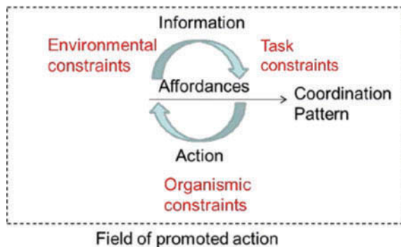
FIGURE 3 Nonlinear pedagogy: introducing constraints into a field of promoted action. The inclusion of different constraints affects the recurrent perception–action loops of the organism–environment dynamical system, bringing forth new affordances for performing a specific task-oriented coordination pattern. Adapted from Newell (1996).
