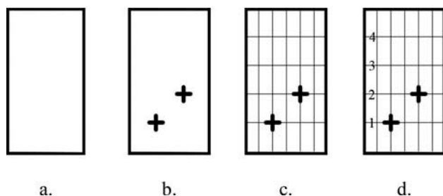
FIGURE 2 Mathematical Imagery Trainer for Proportion display configuration schematics, beginning with (a) a blank screen and then featuring a set of virtual objects overlaid incrementally by the facilitator onto the display: (b) cursors, (c) a grid, and (d) numerals along the y-axis of the grid. For the purposes of this figure, the schematics are not drawn to scale. Also, the actual device enables the tutor to flexibly calibrate the grid, numerals, and target ratio in between trials. The full protocol includes a range of ratios as well as a ratio table.
