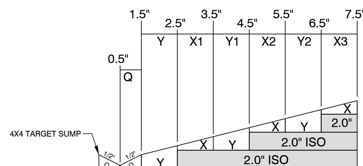
1 PROFILE VIEW OF TAPER 1/4" TAPER SLOPE Scale: NTS
